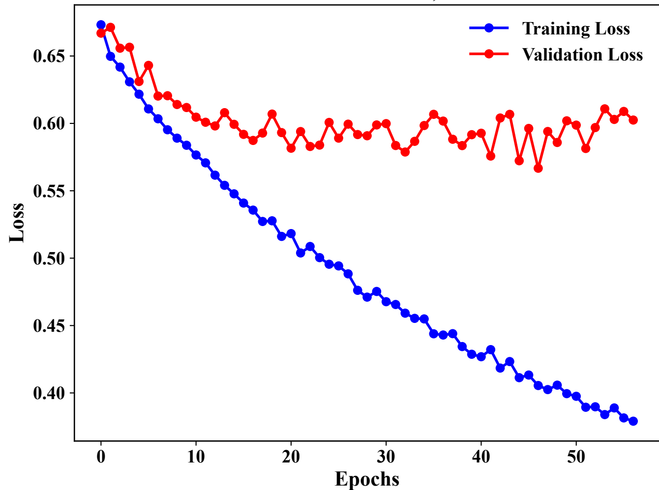
Loss Curves: Seed 64, Rank 2
